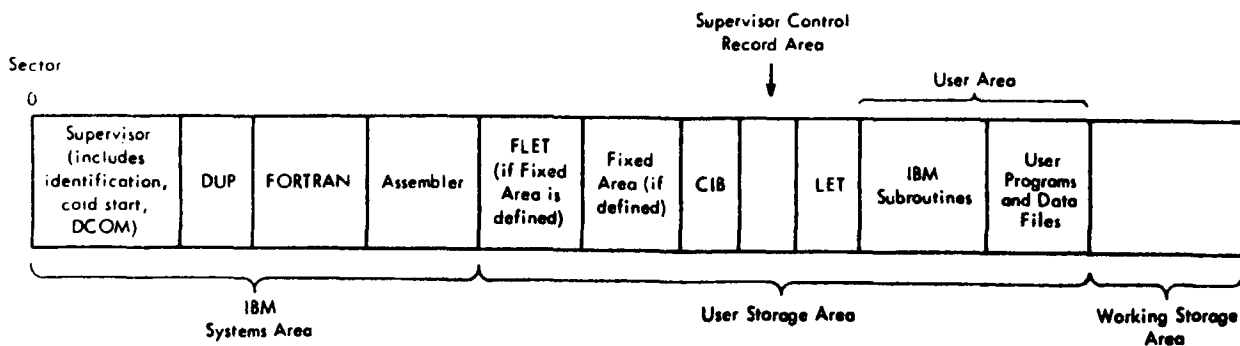
Figure 2. Disk Storage Layout
